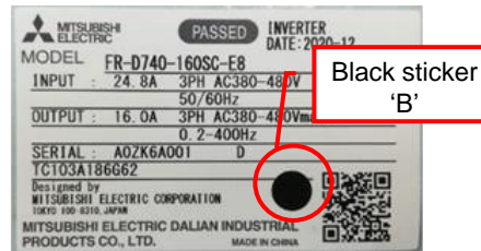
Product serial number plate (over 5.5kW) Repair identified by Black sticker 'B'
